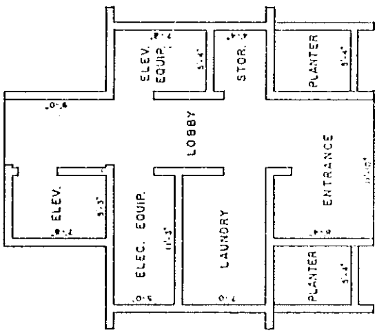
SERVICE CORE DETAIL
